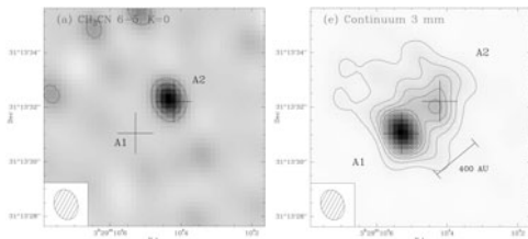
Figure 1. PdB maps of IRAS4A. — (a) CH 3 CN J = 6 - 5, K = 0 line map with 2\sigma contour levels of 16 mJy; (e) 3 mm continuum emission in IRAS4A. The rms and contour levels are 1 and 10 mJy beam -1 respectively. — Crosses show the positions for A1 and A2. The beam size shown in the lower left corner is 1''.1 \times 0''.8 . (Adapted from Bottinelli et al. 2008)
