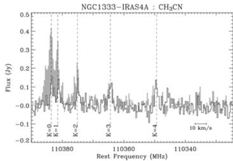
Figure 2. CH 3 CN spectra towards IRAS4A. — Shaded = spectrum obtained at the IRAM 30m Bottinelli et al. 2004; white = Plateau de Bure spectrum averaged over the emission region of IRAS4A2. Dashed lines indicate the frequencies of the CH 3 CN transitions. (From Bottinelli et al. 2008)
