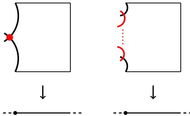
FIGURE 1. The picture shows two kinds of enhancements of the same degenerate central fiber: the red dot on the left stands for [\mathrm{Spec} k/\mu_n] ; on the right we have instead n - 1 extra copies of \mathbb{P}_k^1 wedged between the two branches of the node, also in red.
