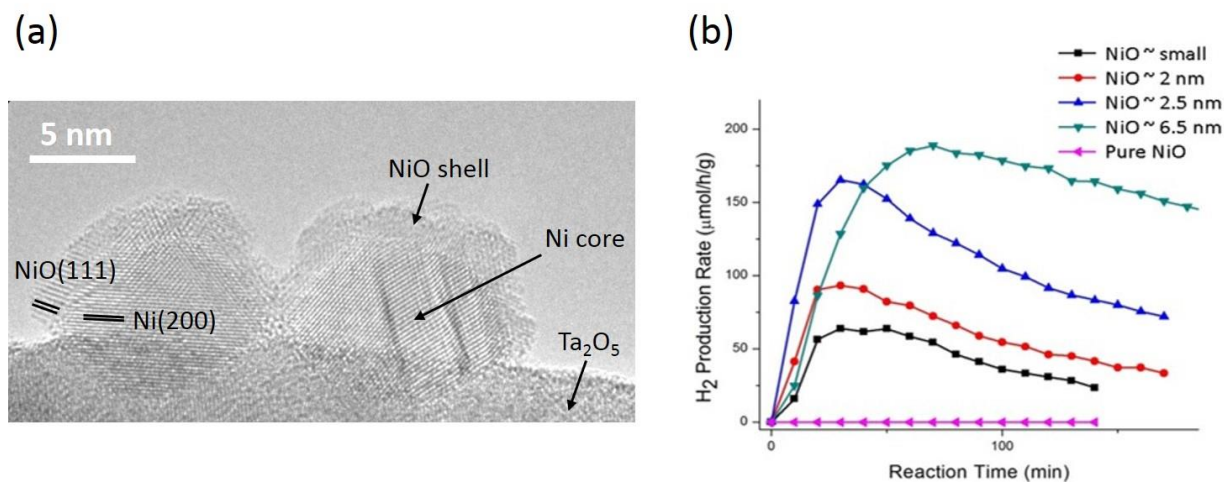
Figure 1. (a) Aberration-corrected TEM image showing a typical Ni core - NiO shell co-catalyst structure. (b) H 2 production rates vs. reaction time of different co-catalysts with a series of NiO shell thickness.
