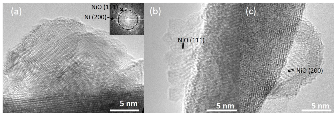
Figure 2. (a) Initial co-catalyst structure which gives the highest H 2 production. FFT indicates both Ni and NiO phases were present initially. After exposure to 16 h UV light and water, two types of deactivated structures emerge: (b) NiO nanoblocks; (c) hollow NiO shell.
