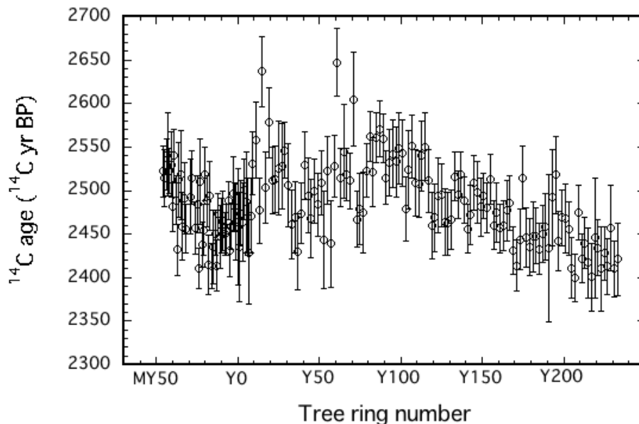
Figure 1 ^{14}\text{C} ages of 165 single-year tree rings in the Choukai Jindai cedar measured by AMS
