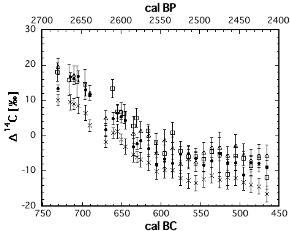
Figure 6 Time profiles of \Delta^{14}\text{C} for the Choukai_AMS data (filled circles), the Belfast data (open triangles), the Seattle data (open squares), and SHCal04 Southern Hemisphere calibration data (crosses).
