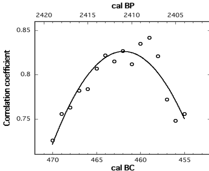
Figure 3 Most probable calendar date of Y233 calculated by the correlation coefficient (open circles) between the Choukai_AMS and IntCal04 data sets. A least-squares-fitted quadratic function (solid line) indicates a maximum at 462 cal BC (2411 cal BP) for Y233.
