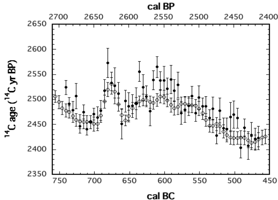
Figure 4 Time profiles of ^{14}\text{C} ages for the Choukai_AMS (closed circles) and IntCal04 (open circles) data sets. The Choukai_AMS data set consists of weighted averages for single-year data adjusted to the 5-yr spans of IntCal04, with Y233 defined as 462 cal BC.
