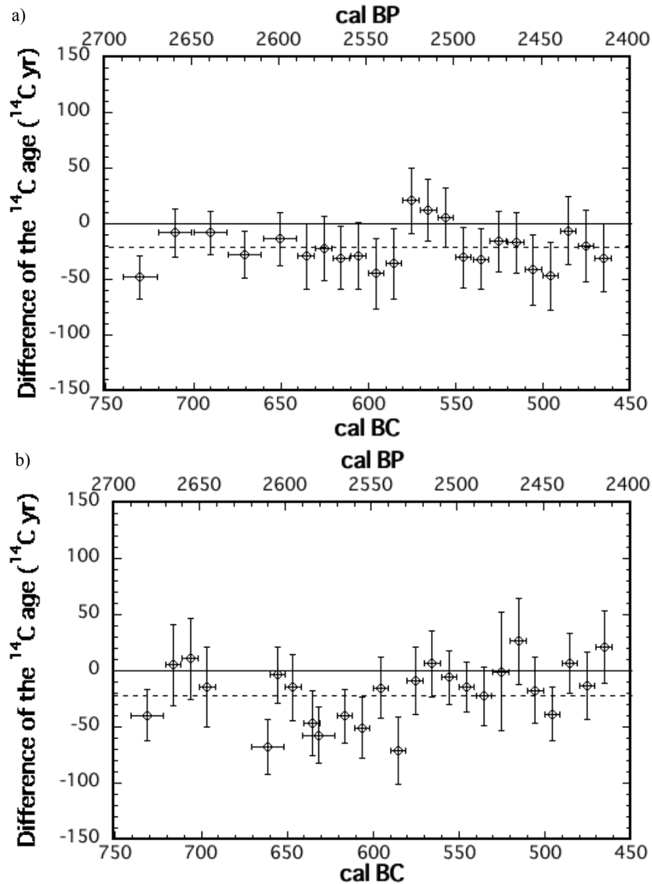
Figure 5 a) Time profiles of the ^{14}\text{C} age difference between the Belfast and Choukai_AMS data sets. The weighted average of the ^{14}\text{C} age difference was -21.3 \pm 5.5 ^{14}\text{C} yr (dashed line). b) Time profiles of the ^{14}\text{C} age difference between the Seattle and Choukai_AMS data sets. The weighted average of the ^{14}\text{C} age difference was -22.7 \pm 5.6 ^{14}\text{C} yr (dashed line).
