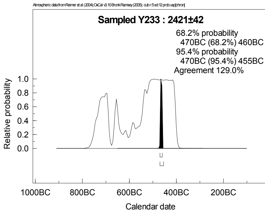
Figure 2 Most probable calendar date of tree-ring number Y233 calculated by OxCal v 3.10 for the IntCal04 calibration curve; 470–455 cal BC is equivalent to 2419–2404 cal BP.
