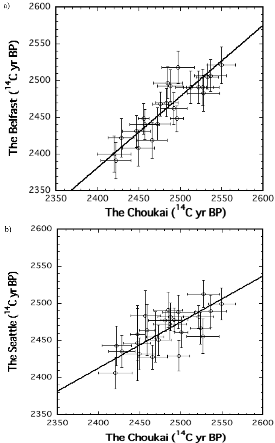
Figure 7 a) Scatter plot for the Choukai_AMS and Belfast data sets. The gradient of the least-squares-fitted line is 0.97 \pm 0.16 . b) Scatter plot of the Choukai_AMS and Seattle data sets. The gradient of the least-squares-fitted line is 0.62 \pm 0.14 .
